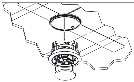
Figure 2. New construction bracket
