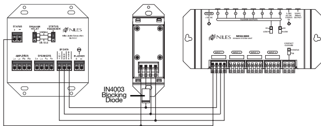
Figure 5: An IR sensor cable is “daisy-chained” from an IntelliPad, to a sensor and back to the MSU480.
