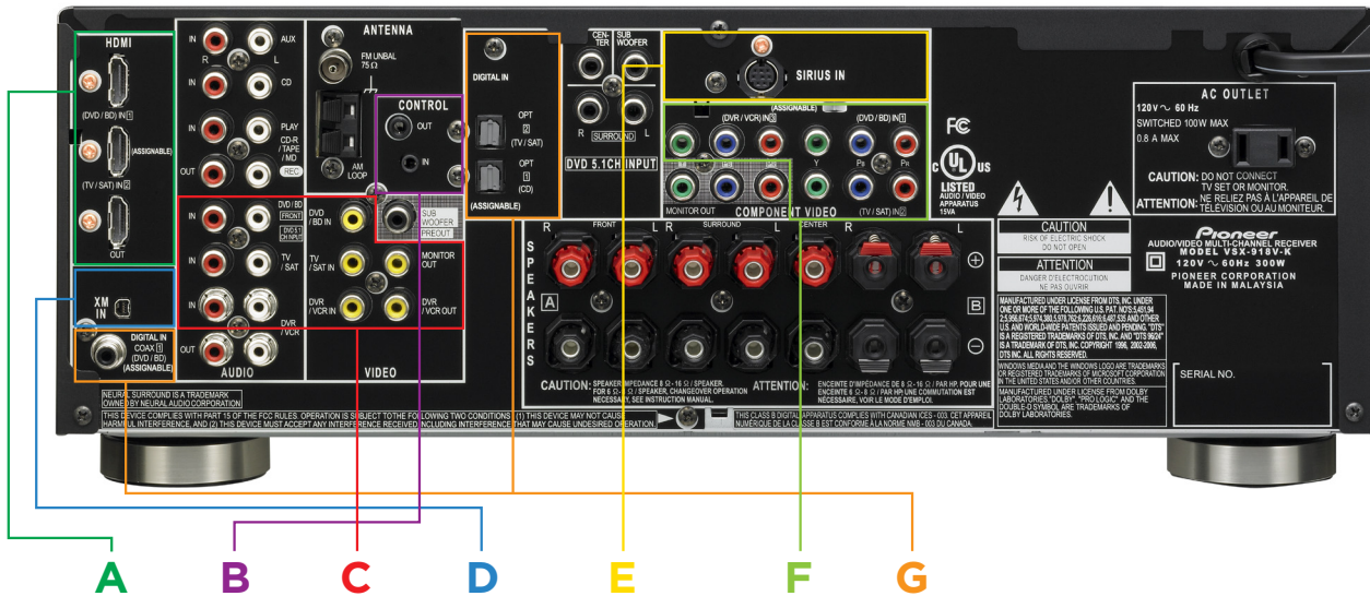
Rear Panel
